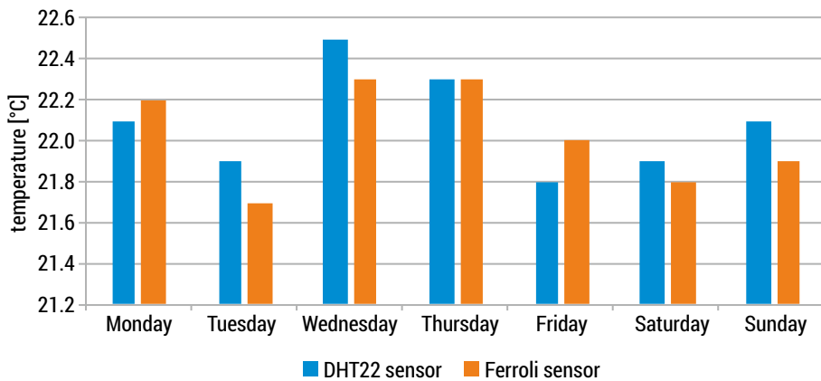
FIGURE 2.9. A graph comparing the average daily room temperature of the DHT22 sensor and the Ferroli sensor over 7 days
