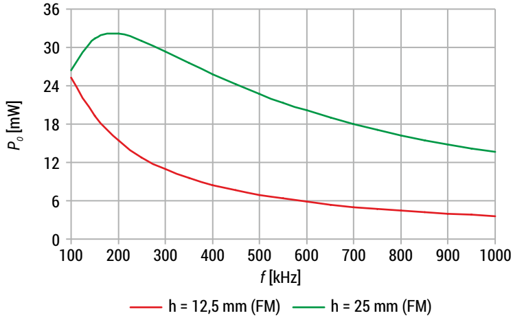
FIGURE 5.5. Results of receiver power ( P_o ) dependent on the distance at number of turns ( n = 90 )
