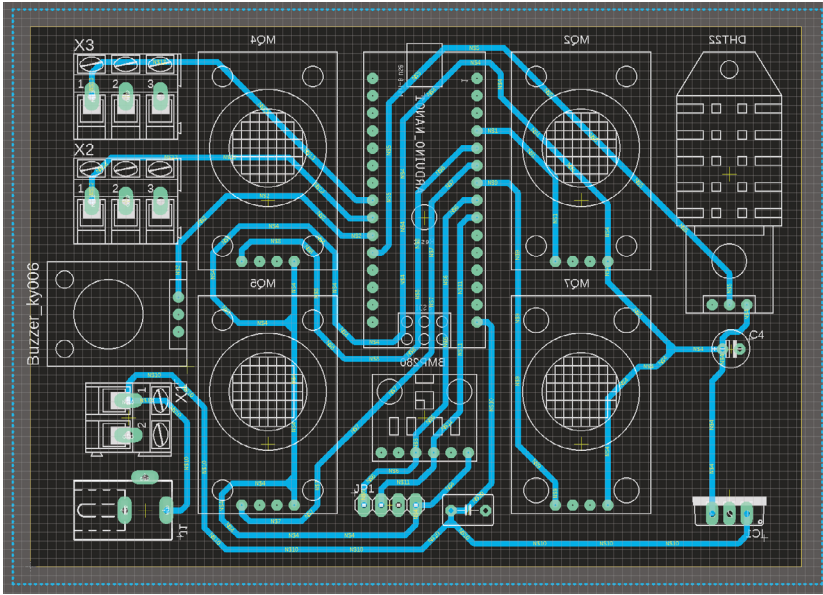
FIGURE 2.3. Visualization of the PCB with connections between system components
