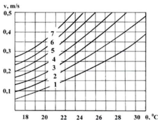
Fig. 8.1. The operation zone air flow characteristics, where: v – maximal air velocity, m/s; \theta – the air temperature at the measuring point, 1–7 – air characteristics (Source: STR1, 2005)
