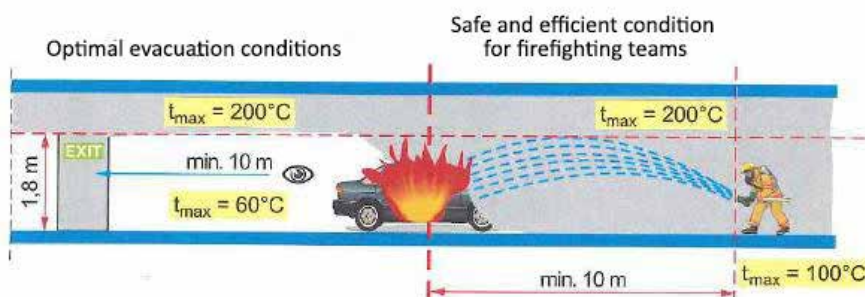
Fig. 9.2. Acceptable conditions for firefighting in a garage depending on the purpose of system operation (Source: based on data from ALNOR, 2017; Mizielirski & Kubicki, 2012)
