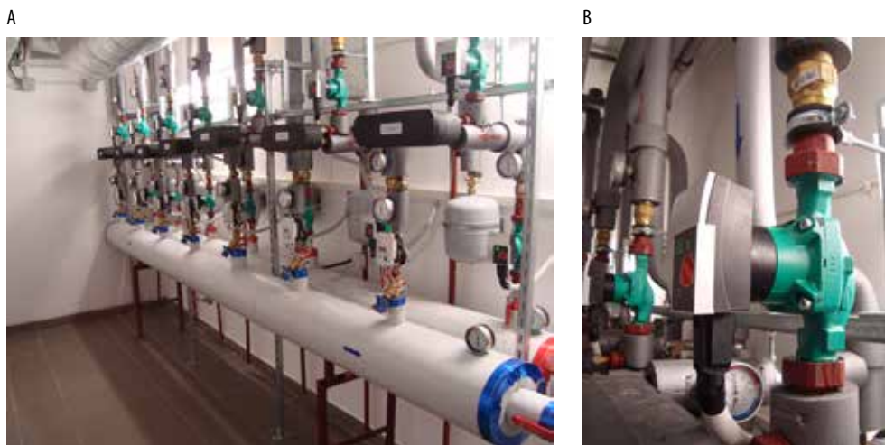
Fig. 7.19. Circulation pumps in a boiler room (Source: photos by T.J. Teleszewski)
