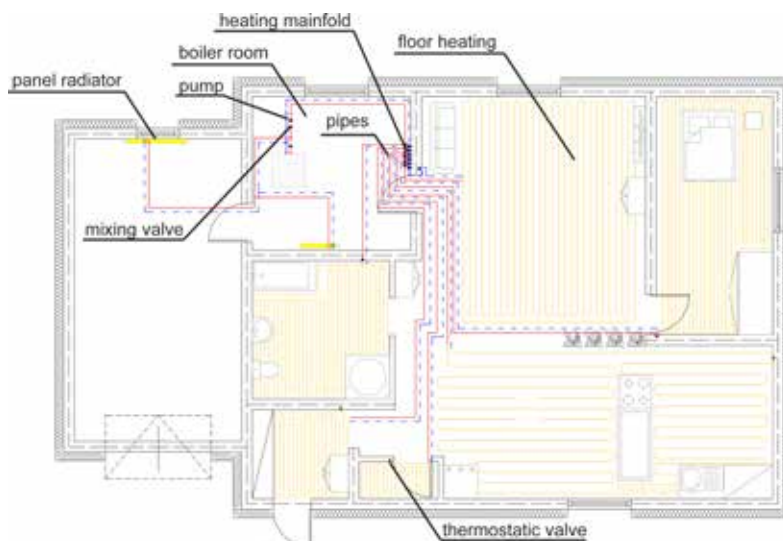
Fig. 7.1. Main components of a heating system. A) Schema, B) Example of heating system in a house (Source: own elaboration)
