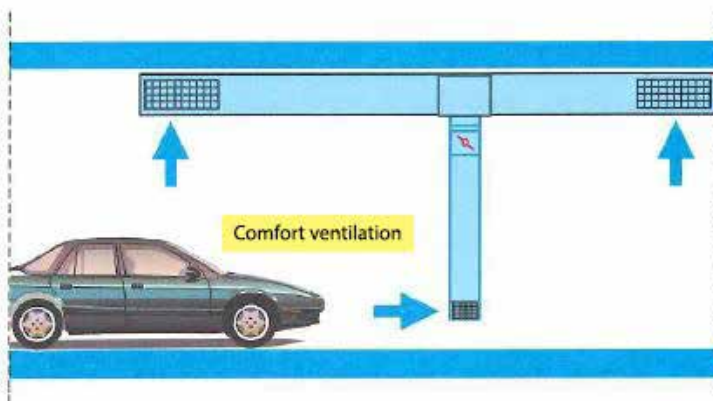
Fig. 9.7. Operation of the duct ventilation system in normal conditions (Source: based on data from ALNOR, 2017; WEB-1)
