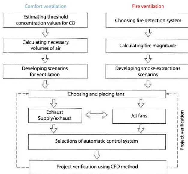
Fig. 9.13. Design procedure for ductless system (Source: based on data from ALNOR, 2017; Mizieliński & Kubicki, 2012)
