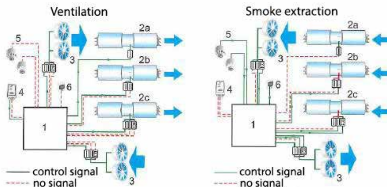
Fig. 9.12. Control of the ventilation system in home and fire ventilation (Source: based on data from ALNOR 2017, Król 2014)
